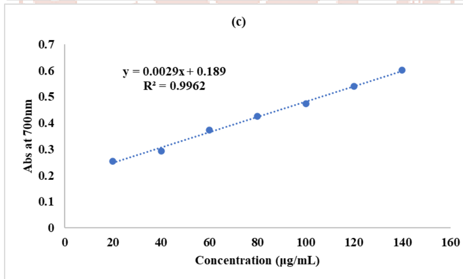
Figure 1: Standard graph of (a) gallic acid for total phenol estimation, (b) quercetin for total flavonoid estimation, and (c) tannin acid for total tannin estimation for quantitative analysis of E. alba .
