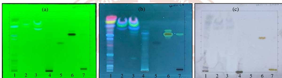
Figure 2: HPTLC chromatogram of E. alba : (a) 254nm; (b) 366nm and (c) anisaldehyde-H 2 SO 4 derivatization, with tracks (1) E. alba methanolic extract; (2) E. alba petroleum ether extract; (3) E. alba toluene extract; (4) E. alba water extract; (5) gallic acid; (6) quercetin and (7) rutin.
