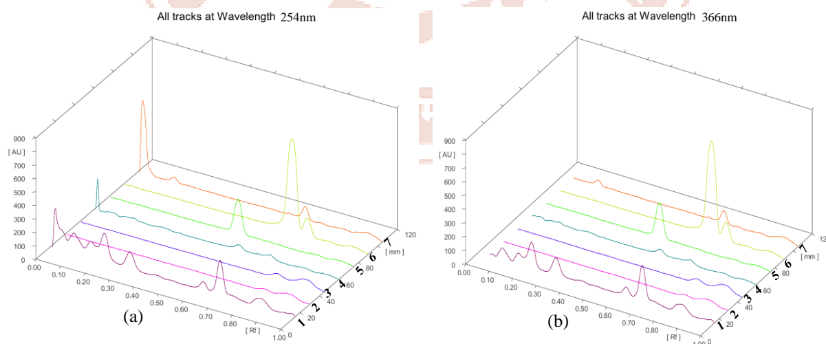
Figure 3: HPTLC Densitograms of E. alba samples and standards, all tracks at wavelength (a) 254nm and (b) 366nm with track (1) E. alba methanolic extract; (2) E. alba petroleum ether
